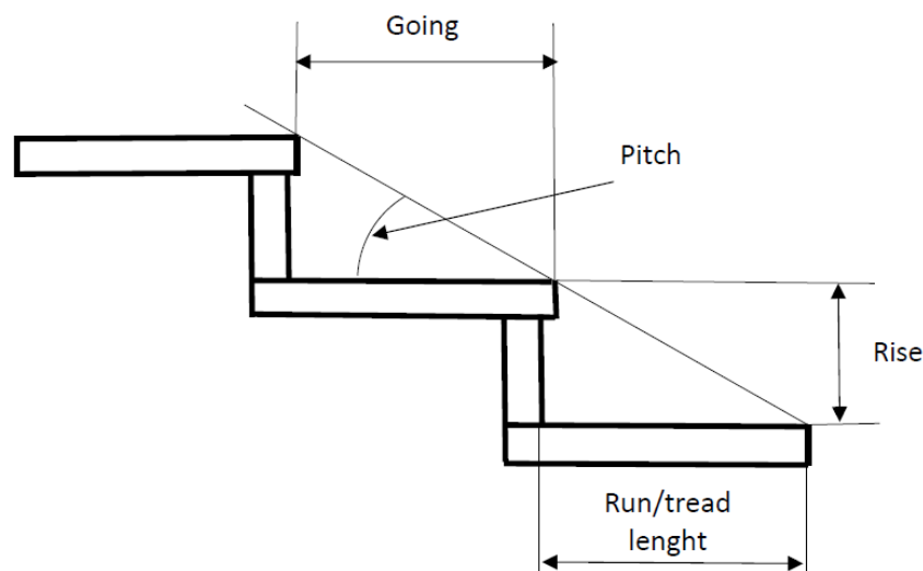
Figure 3: Schematic diagram of stair terminology. Source: (Scott, 2005) (Komisar, V., McIlroy, W.E., and Duncan, C.A., 2019)
