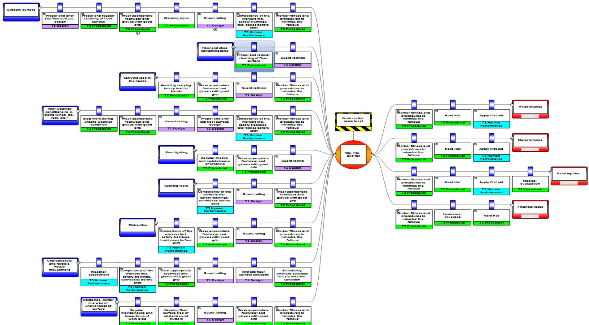
Figure 13: Bowtie diagram of STF for work on the same level. Source: (Komisar, V., McIlroy, W.E., and Duncan, C.A., 2019) (Hanson, J. P., Redfern, M. S., and Mazumdar, M., 2010) (Chang, W., Leclercq, S., Lockhart, T. & Haslam, R., 2016) (Appendix 2: Pre-test questionnaire)
